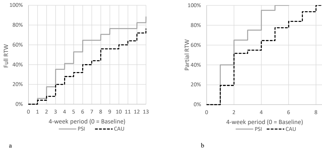
Supplemental Figure 2. (a) Kaplan-Meier curve showing the part of the groups that had fully returned to work measured over the 12-month follow-up period. (b) Kaplan-Meier curve showing the part of the groups that partially returned to work measured over the 12-month follow-up period. PSI = Problem-Solving Intervention; CAU = Care As Usual
