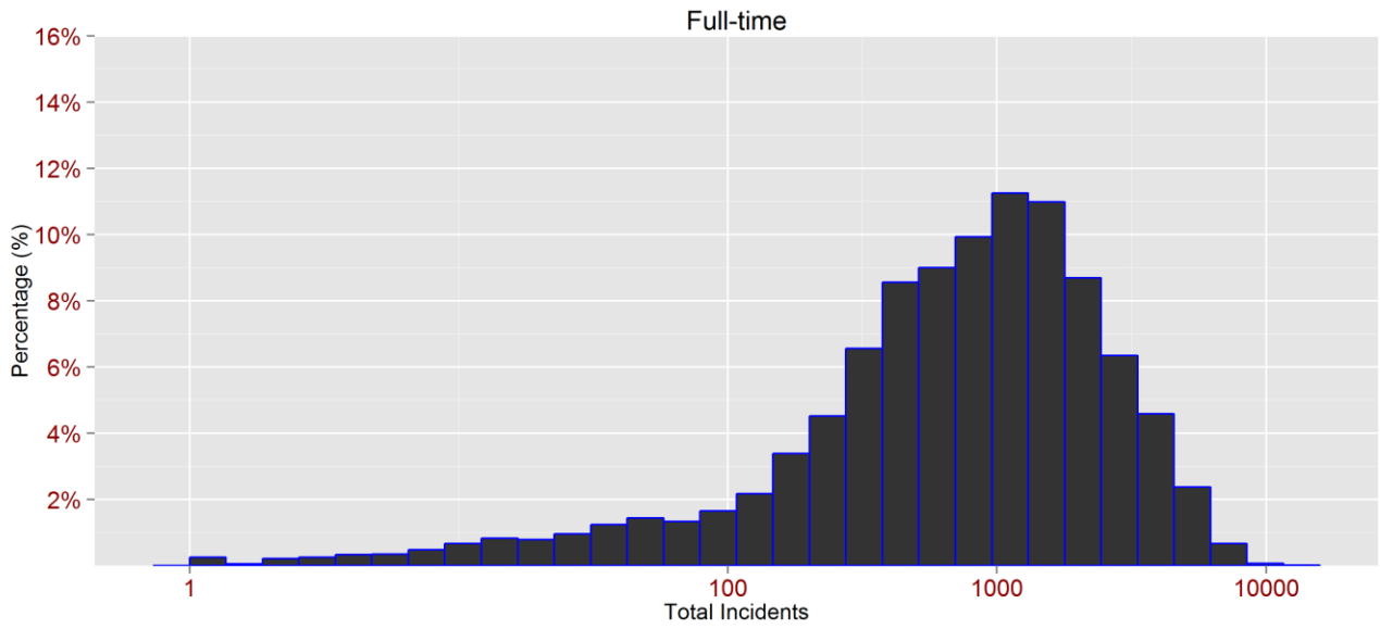
Supplementary Figure 1 Distribution of the number of incidents attended by individual full-time and part-time firefighters on a log scale
